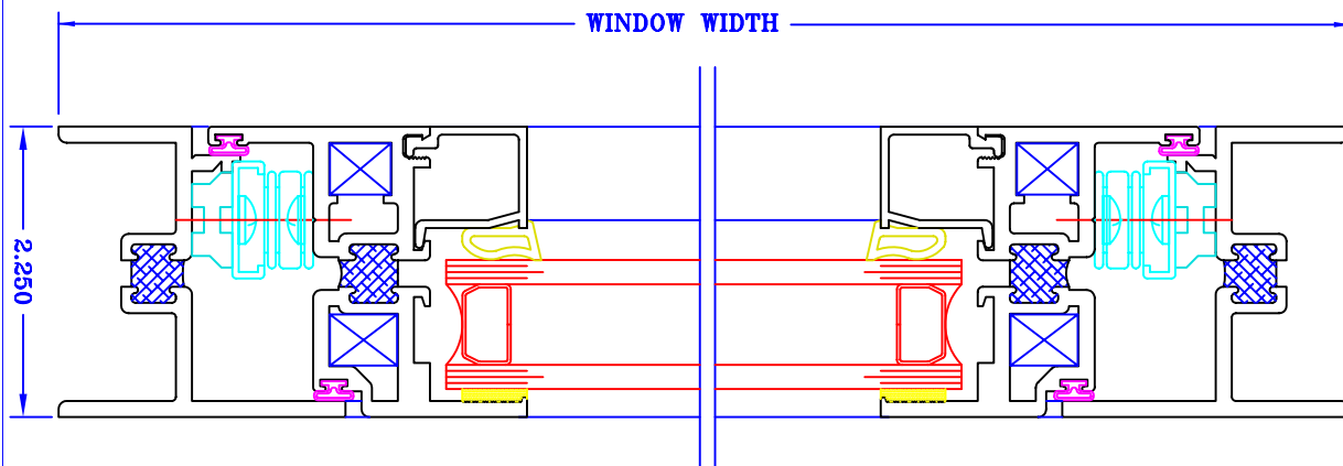
ALUMINUM PROJECT IN Series #CTC-8300 TOP VIEW (1:1)
