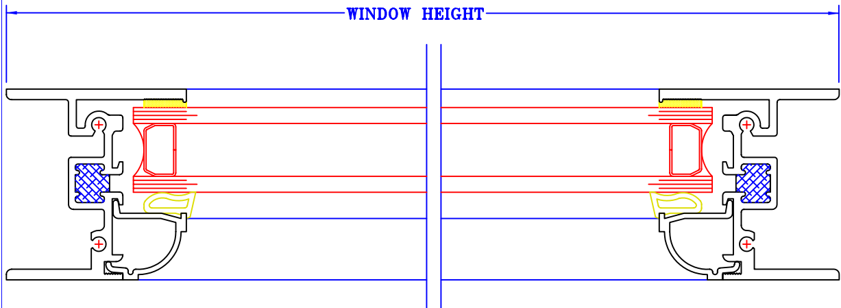
ALUMINUM PICTURE Series #CTC-8100 SIDE VIEW (1:1)
