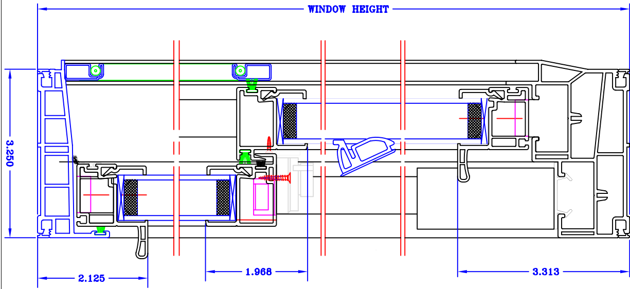
FULLY WELDED VINYL WINDOW REPLACEMENT DOUBLE HUNG TILT #CVD-500 SIDE VIEW (1:1)
