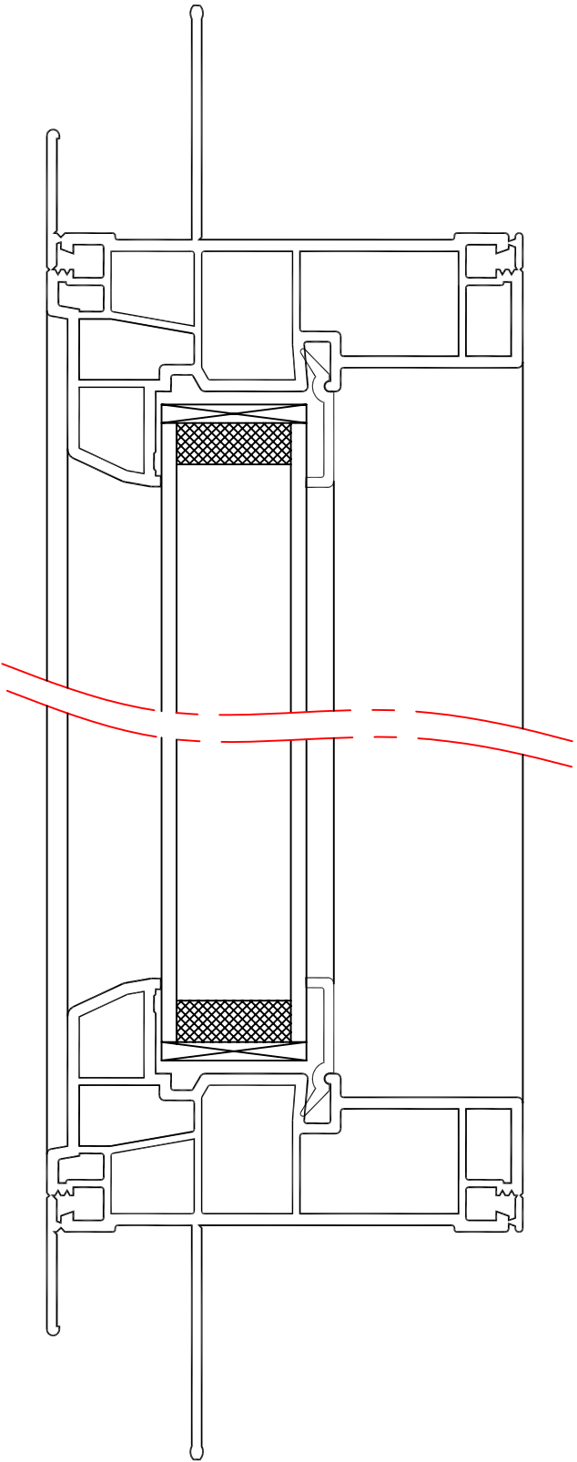
FULLY WELDED VINYL WINDOW NEW CONSTRUCTION PICTURE #CVP-410B w/ BRICK MOLD TOP / SIDE VIEW (1:1)
