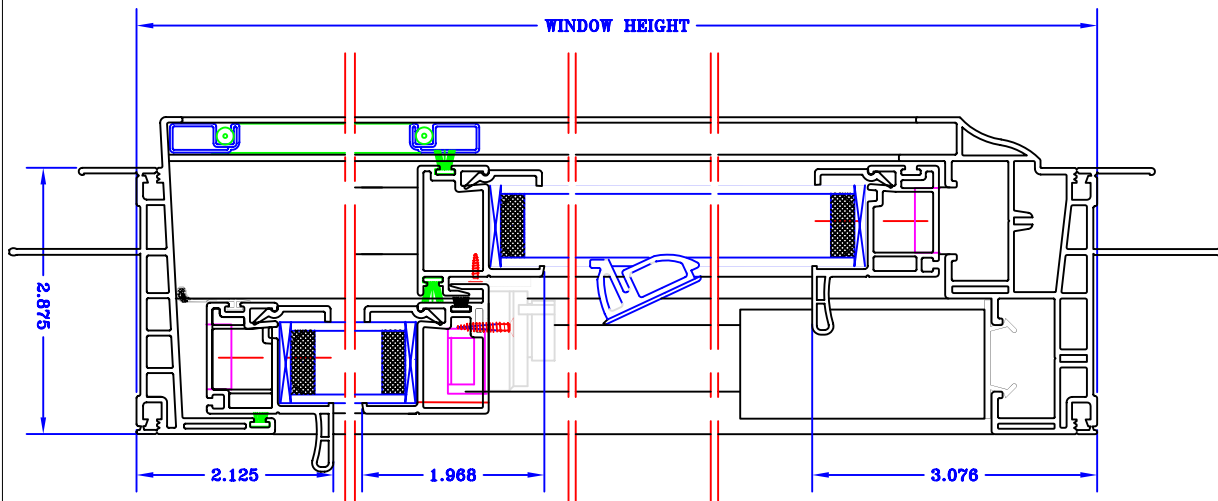
FULLY WELDED VINYL WINDOW NEW CONSTRUCTION DOUBLE HUNG TILT #CVD-400 SIDE VIEW (1:1)
