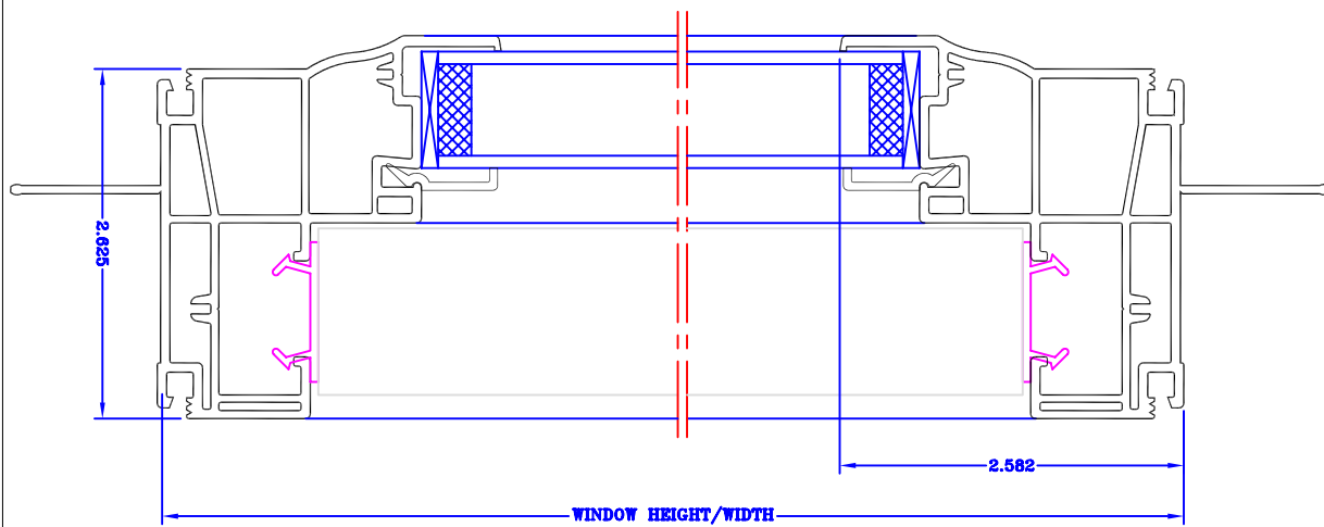
FULLY WELDED VINYL WINDOW NEW CONSTRUCTION PICTURE #CVS-310 1:1
