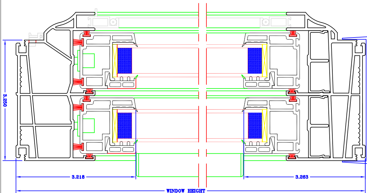
FULLY WELDED VINYL WINDOW SLIDER #CVS-220 SIDE VIEW (1:1)
