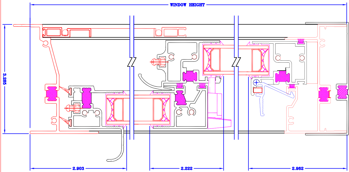
THERMAL BREAK ALUMINUM WINDOW DOUBLE HUNG TILT #CTD-2000 SIDE VIEW (1:1)
