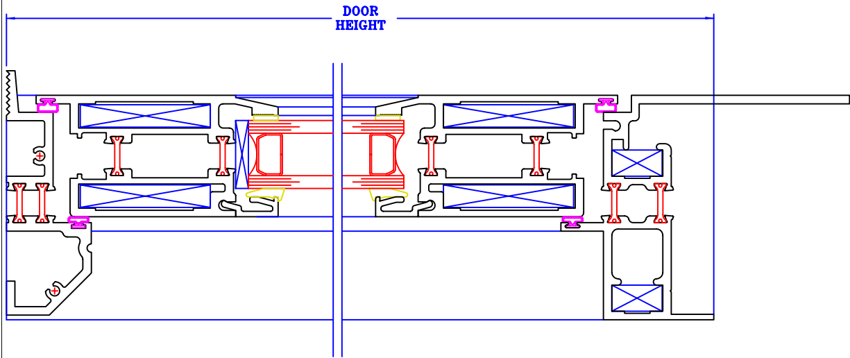
THERMAL BREAK ALUMINUM TERRACE DOOR #CTT-1400 SIDE VIEW (1:1)
