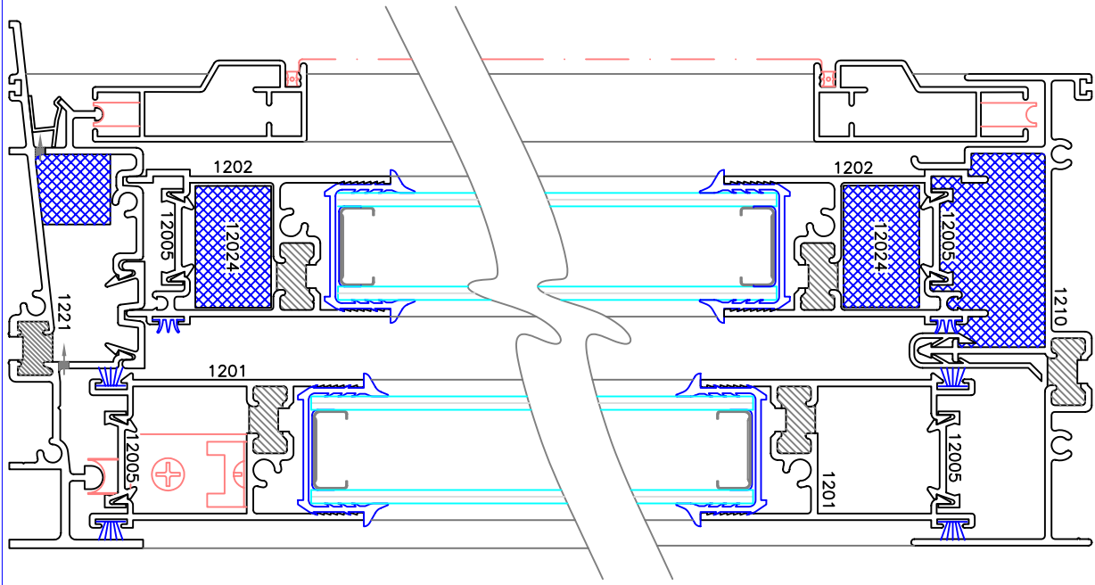
ALUMINUM PATIO SLIDING DOOR #CTP-1200 SIDE VIEW (1:1)
