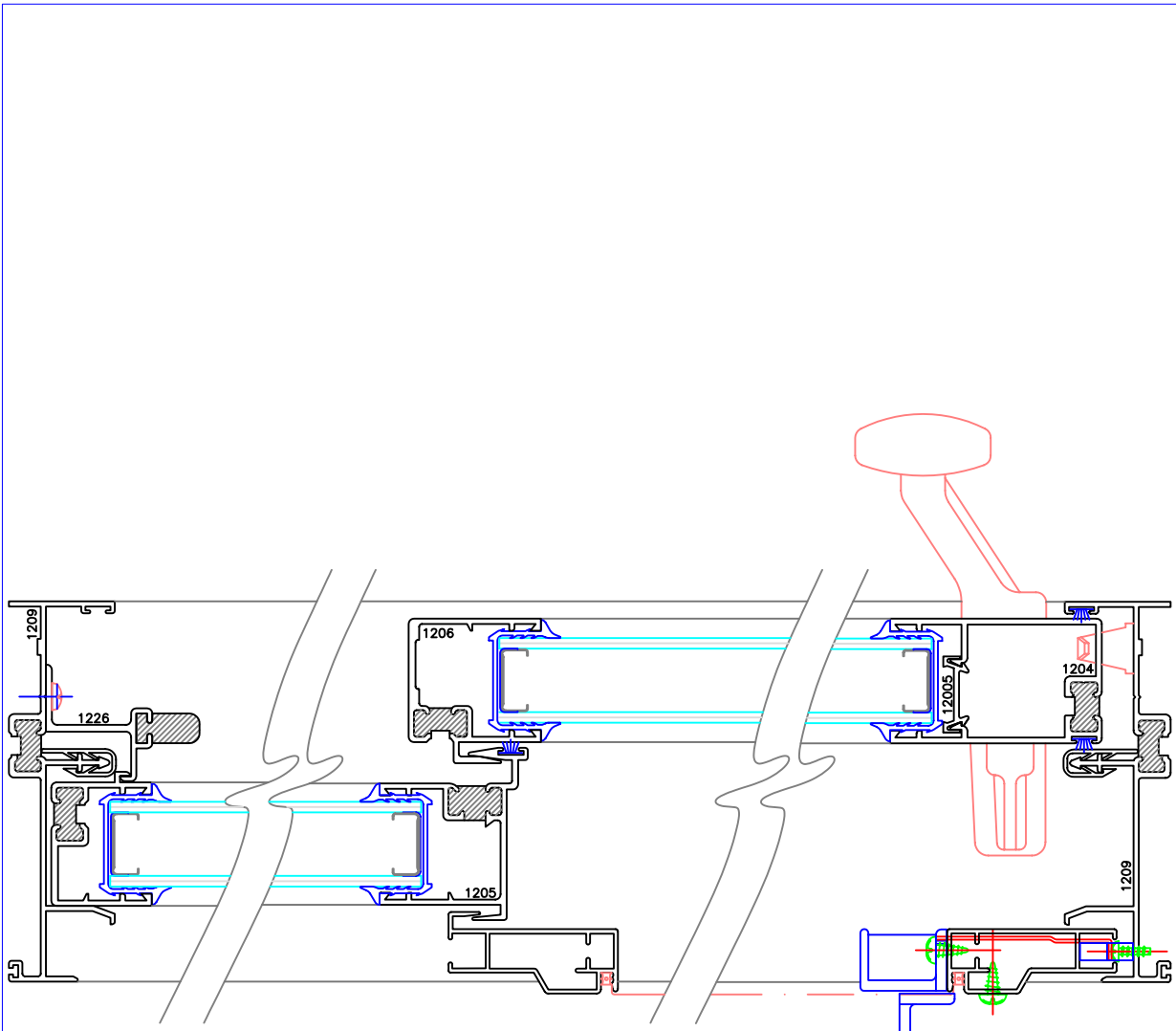
ALUMINUM PATIO SLIDING DOOR #CTP-1200 TOP VIEW (1:1)
